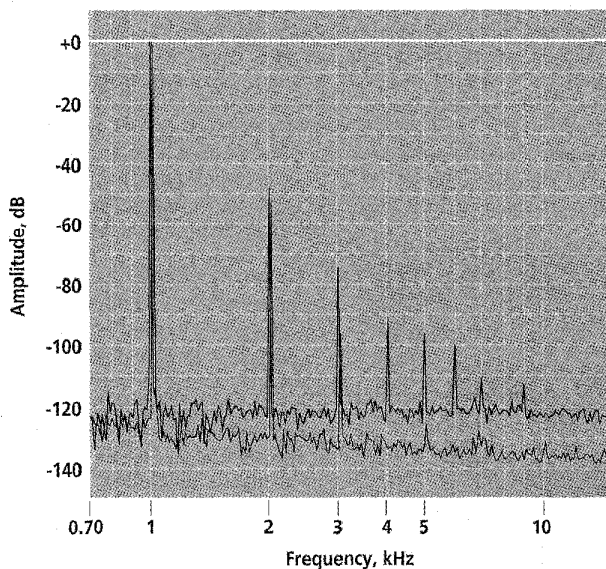
6AU6A pentode: Noise floor is about 120 dB below the fundamental; second harmonic is 48 dB down [red curve, above]. Operating conditions were taken from the resistance-coupled amplifier tables in RCA tube manual RC-21, 1961, p. 438.
