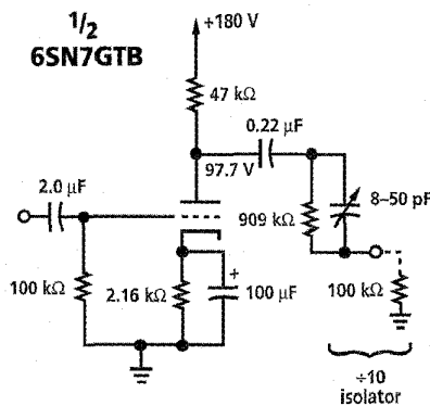
6SN7GTB medium-mu triode: Noise floor is about 130 dB below the fundamental; second harmonic is 52 dB down [blue curve, above]. Operating conditions were taken from the resistance-coupled amplifier tables in RCA tube manual RC-21, 1961, p. 439. Note: the voltage gain of this device is much lower than that obtained with any of the transistors or the pentode.
